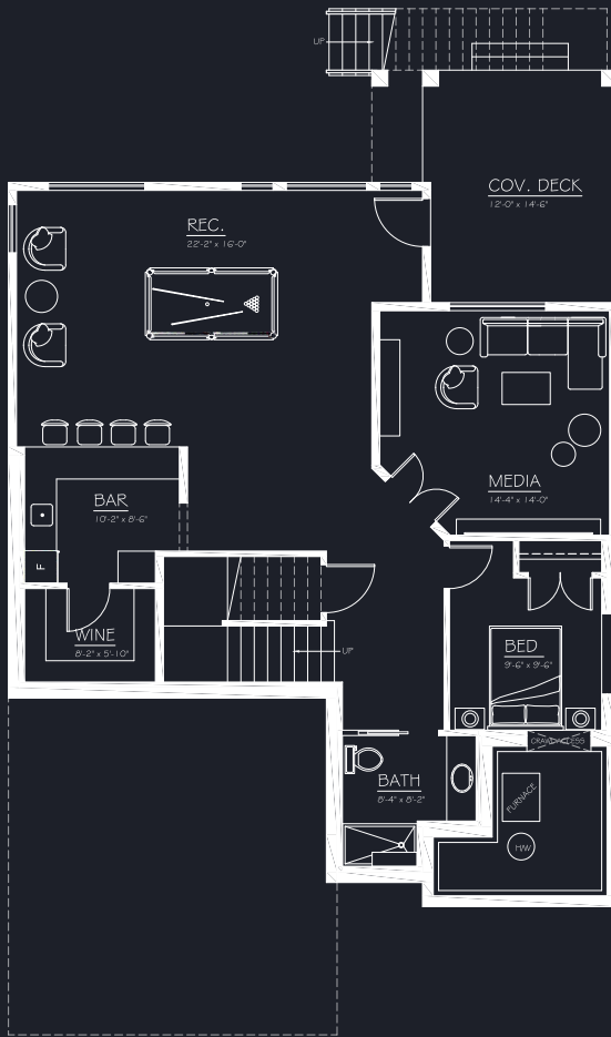
BASEMENT FLOOR - RECREATION LIVING - 1,232.25 sq. ft. CRAWL - 121 sq. ft. TOTAL - 1,353.25 sq. ft.
