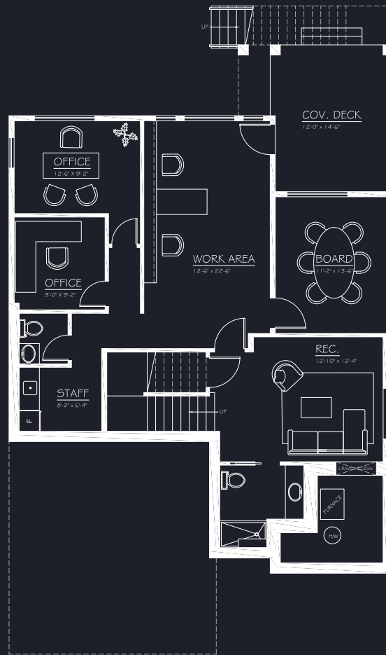
BASEMENT FLOOR - OFFICE LIVING - 392.25 sq. ft. CRAWL - 121 sq. ft. OFFICE - 840 sq. ft. TOTAL - 1,353.25 sq. ft.
